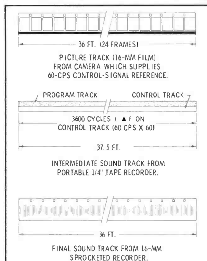
Fig. 5. Relative physical dimensions of elements comprising synchronizing system.
