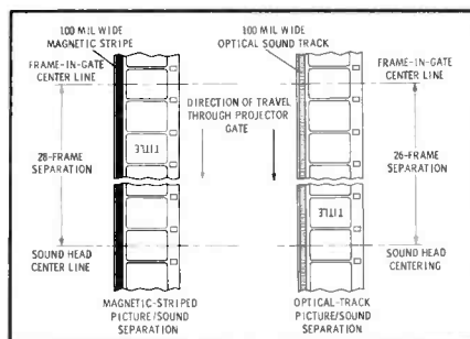
Fig. 1. Relative positions of both picture and sound tracks on final 16mm print film.
