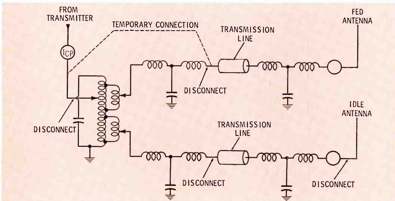
Fig. 2. Modifications made to antenna matching circuit permit feeding power to a remaining tower in a directional array.
