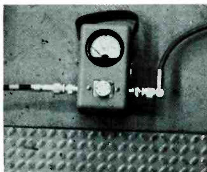
Fig. 4. Wattmeter in typical test setup.
