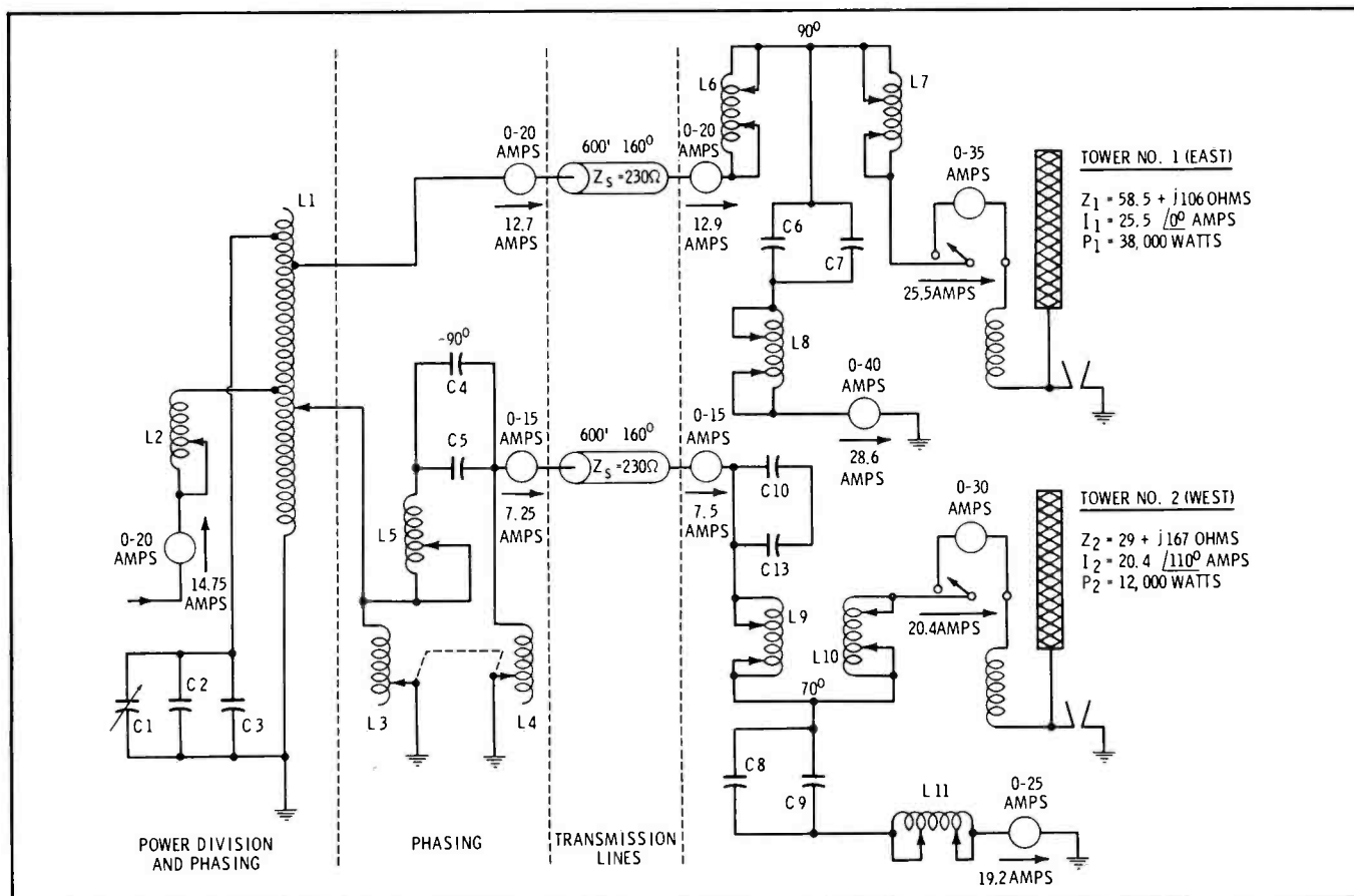
Fig. 2. Antenna tuning, phasing, and power division circuits used at station CKAC.
