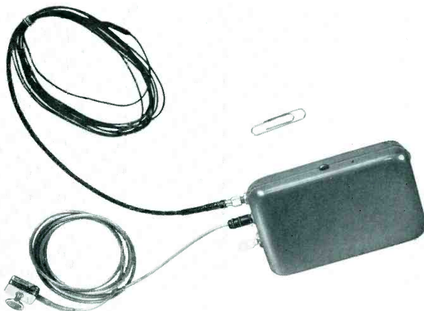
Fig. 3. Typical cigarette-pack-sized transmitter uses buttonhole microphone.
