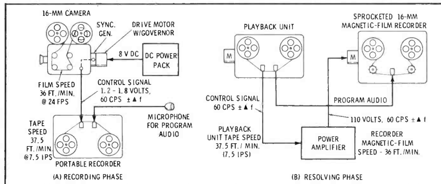
Fig. 6. Hypothetical setup shows function of portable double-system sync equipment.
