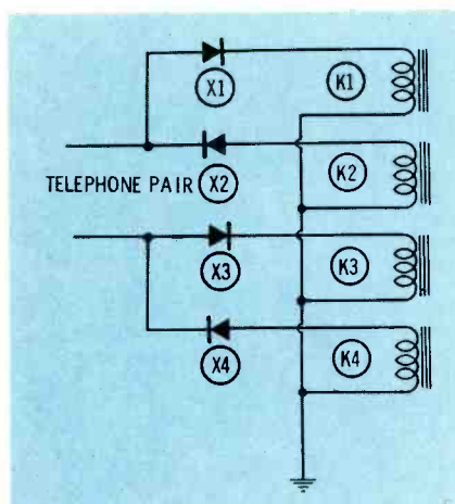
Fig. 1. Basic relay and diode connection.
