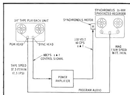
Fig. 2. Power-amplifier resolving method is most direct of the three basic techniques.
